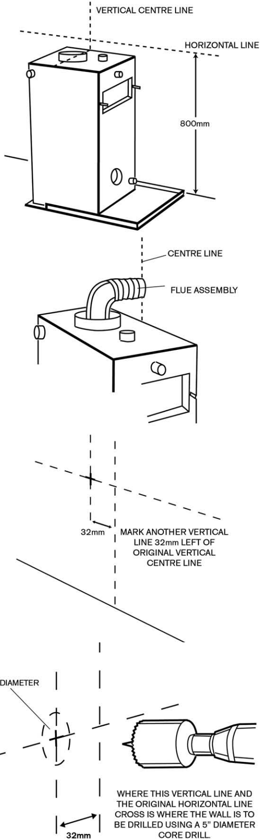
Fig 43 Fitting a RIGHT-HAND balanced-flue
