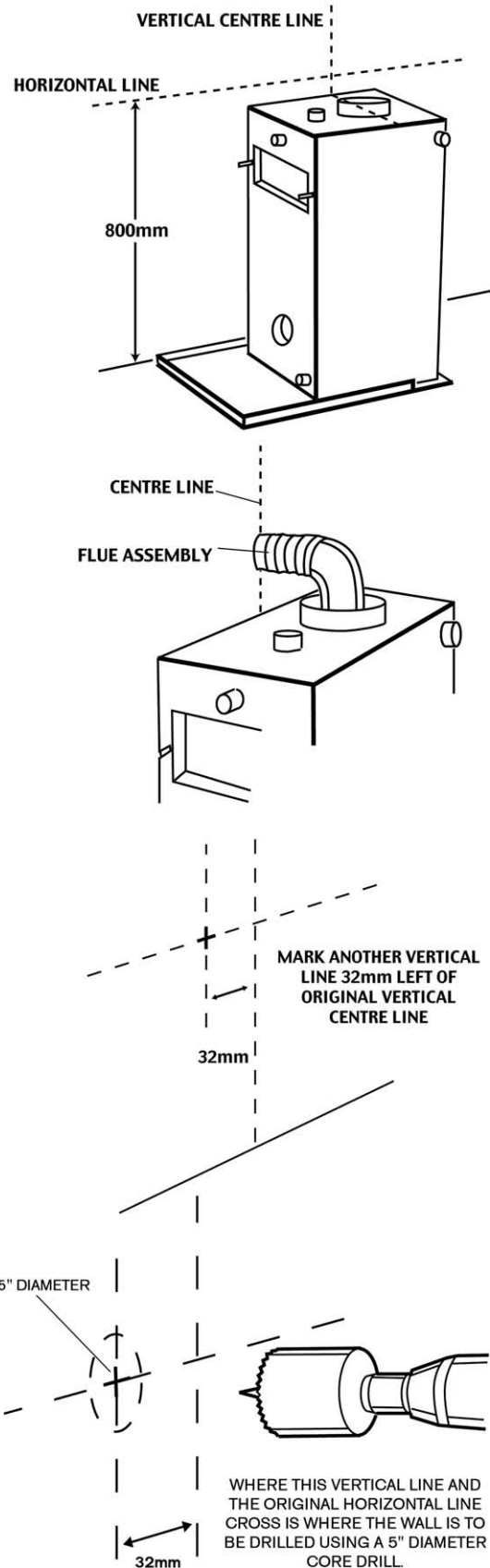
Fig 42. Fitting a LEFT-HAND balanced-flue
