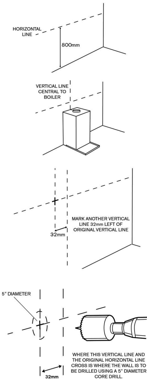
Fig 41 Fitting a REAR balanced-flue
