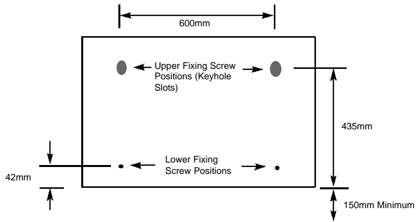
Fig. 5 Marking out Fixing Screw Position
