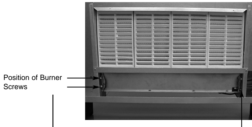
Fig. 10 Burner removal
