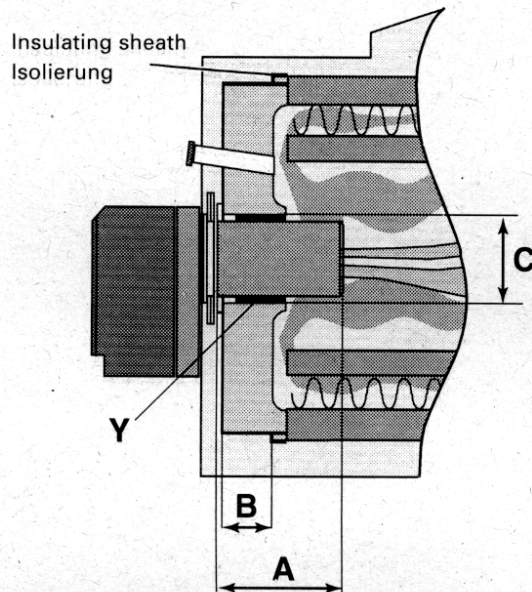
Combustion chamber door - Brennkammertür
